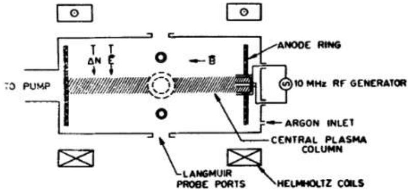
The cross field instability experiment. Radial diffusion from a magnetized central column produces radial density gradient
