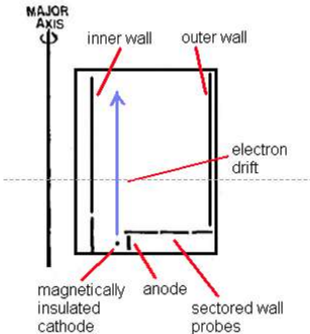
Schematic diagram of the Nonneutral Plasma experiment
