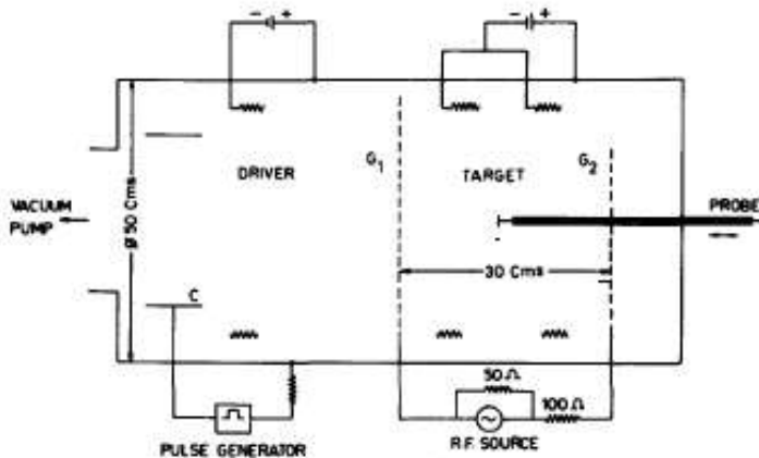
Fig. 1. Schematic drawing of the double plasma machine.
