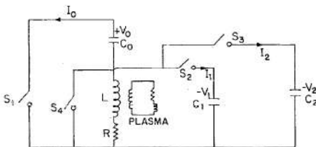
The shaped pulse capacitor bank for plasma discharges in ADITYA
