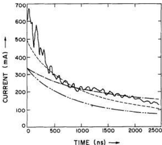
Comparison between the current obtained in (i) experiment (—) (ii) the model (-----) (iii) conduction current (- - -) (iv) model and contribution from the emitted secondary electrons (.....).
